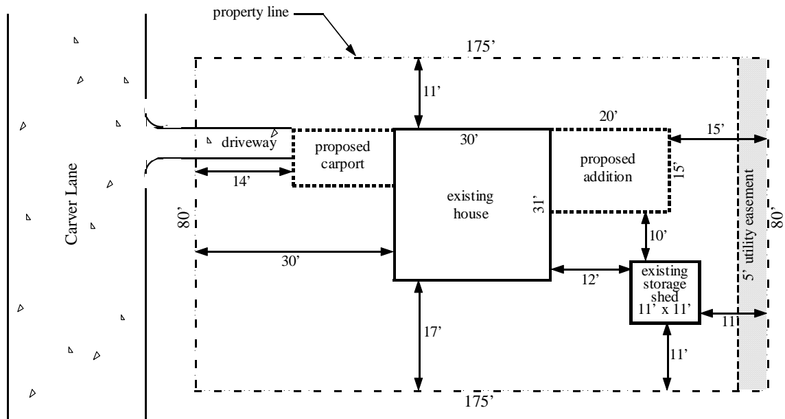
SAMPLE PLOT PLAN
