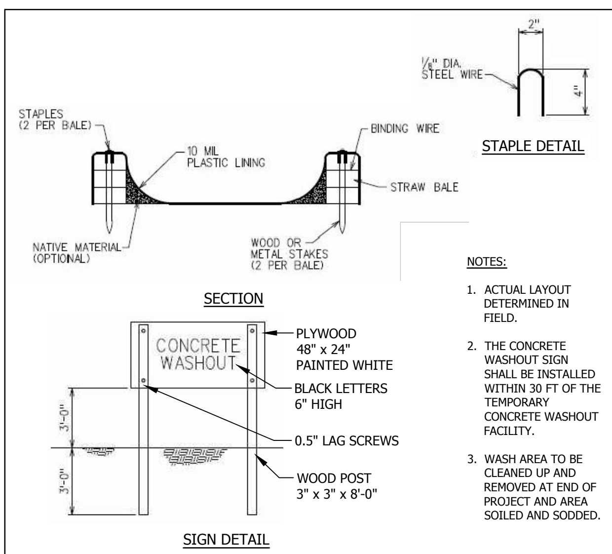
C CONCRETE TRUCK WASH AREA
