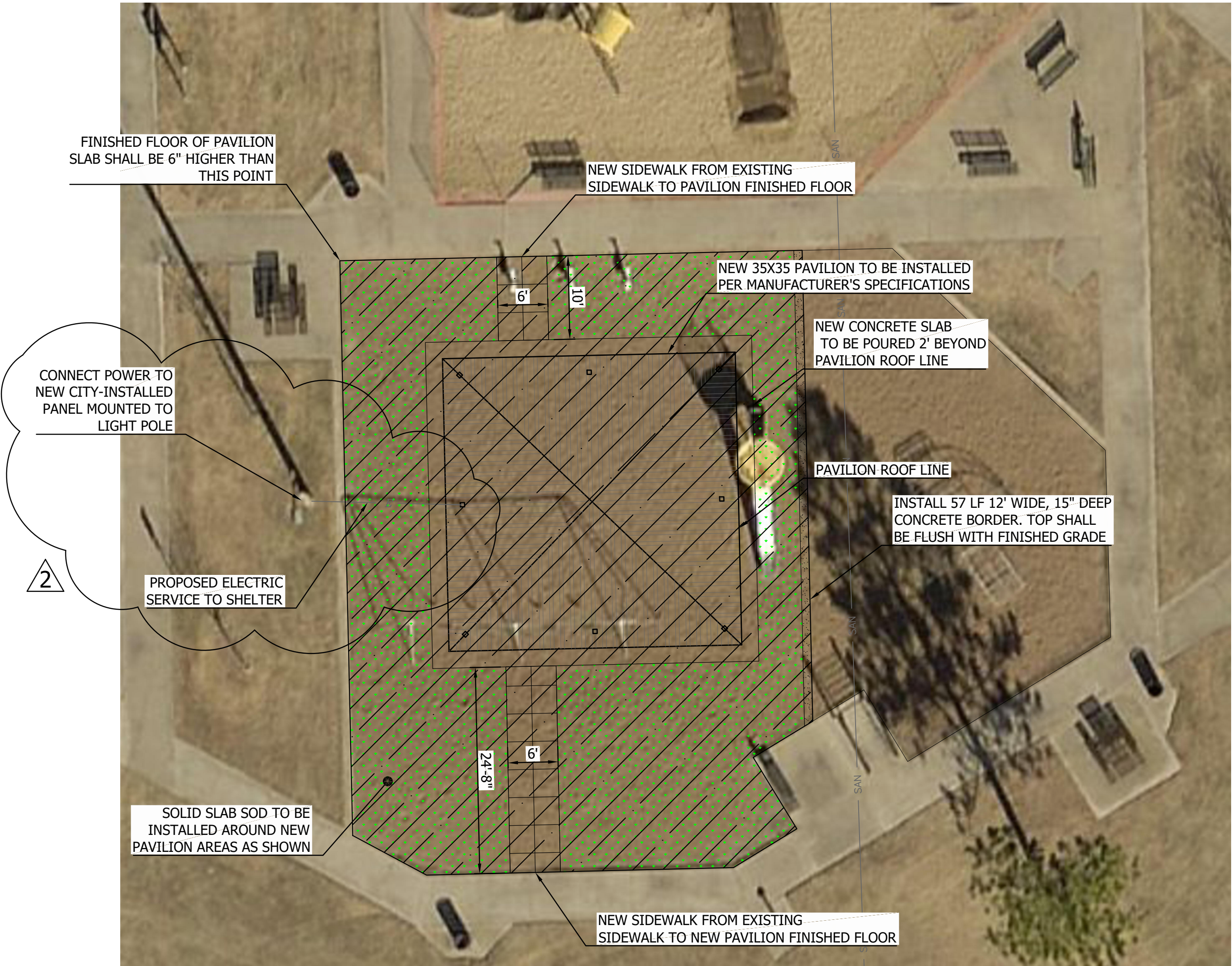
B ENLARGED SITE PLAN 1" = 10'
